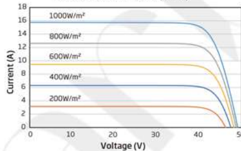
I-V CURVES OF PV MODULE (610W)
